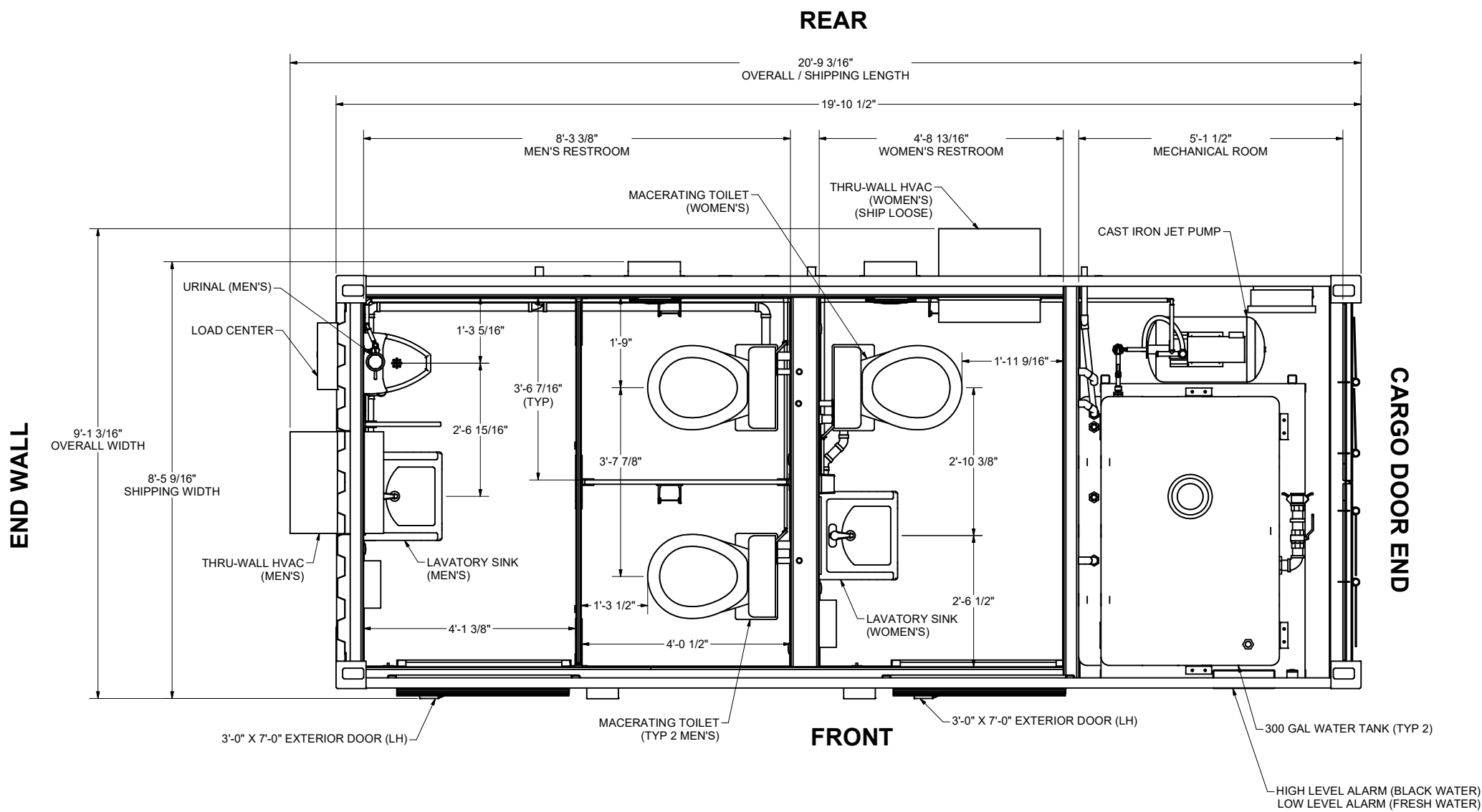
GENERAL ARRANGEMENT - PLAN VIEW SCALE 3/4" = 1'-0"
