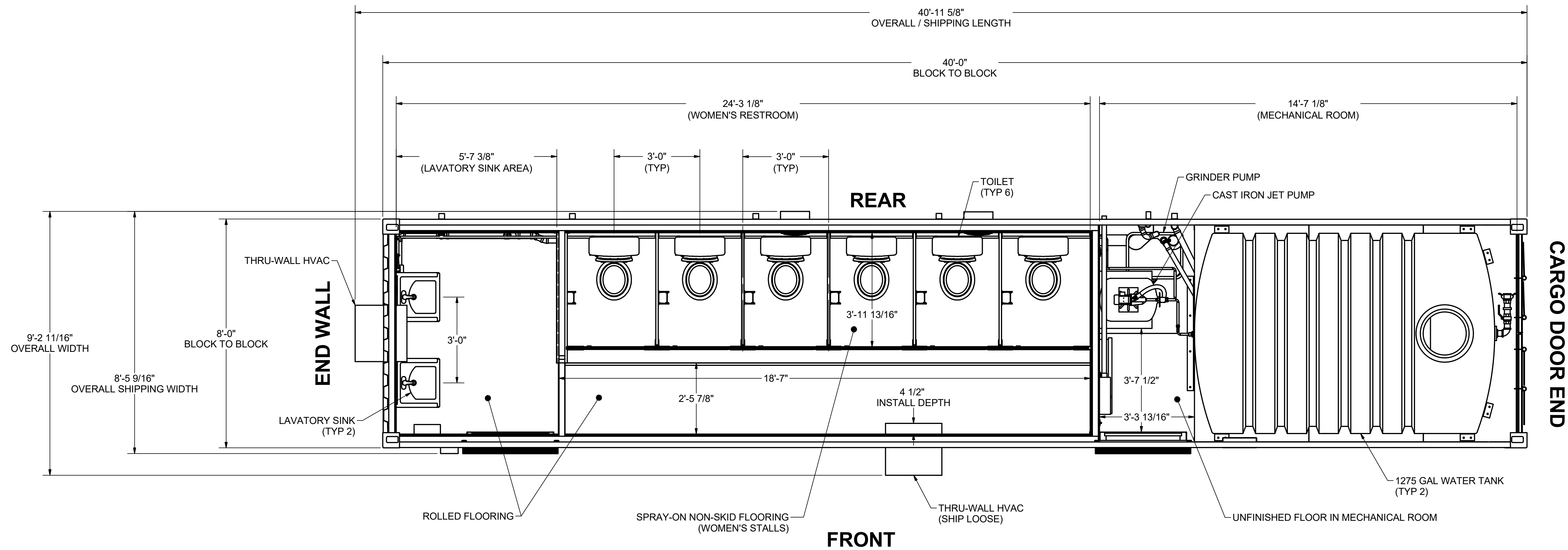
GENERAL ARRANGEMENT - PLAN VIEW SCALE 1/2" = 1'-0"
