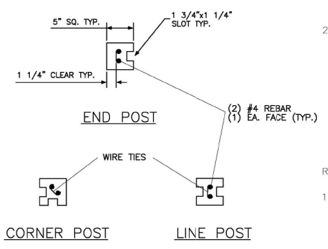
SECTION - 6' SCREENING WALL POST
