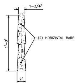
WOODCAST PANEL - SECTION
