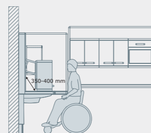
Height adjustment of overhead cupboards
