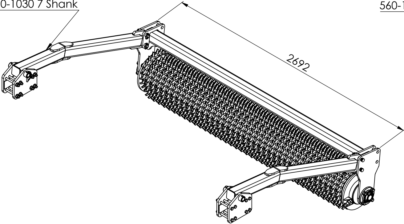
560-1030 7 Shank
