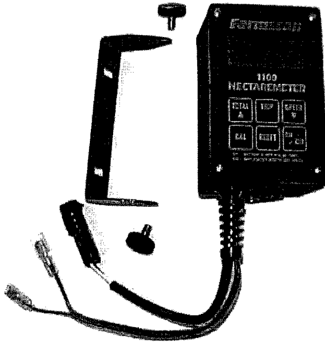
Figure 4.1: Hectaremeter and Mounting Bracket
