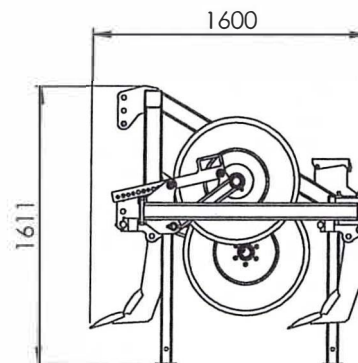
RIGID SHEAR PIN RECOIL SHANKS WITHOUT COULTERS
