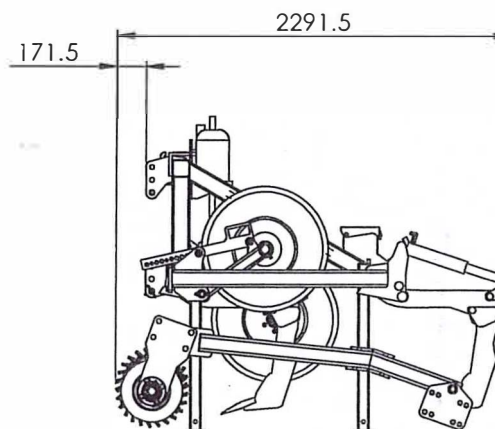
MOUNTED FLEXIROLLER AT FRONT SUITS HYDRAULIC SHANKS
