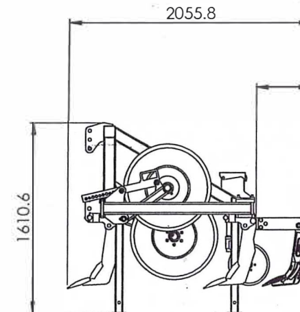
RIGID SHEAR PIN RECOIL SHANKS WITH COULTERS
