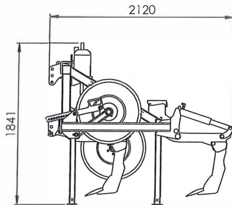
HYDRAULIC RECOIL SHANKS WITH OR WITHOUT COULTERS
