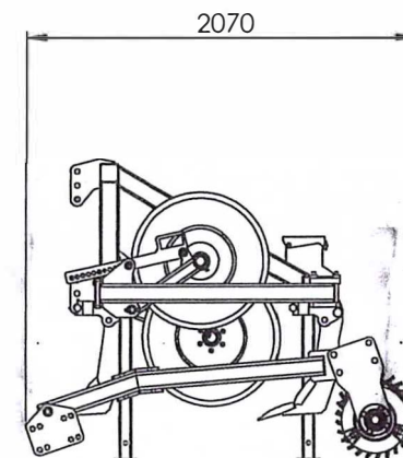
MOUNTED FLEXIROLLER AT BACK SUITS RIGID SHANKS
