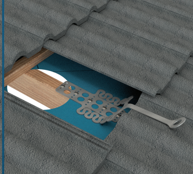
Tiled Roof Anchor
