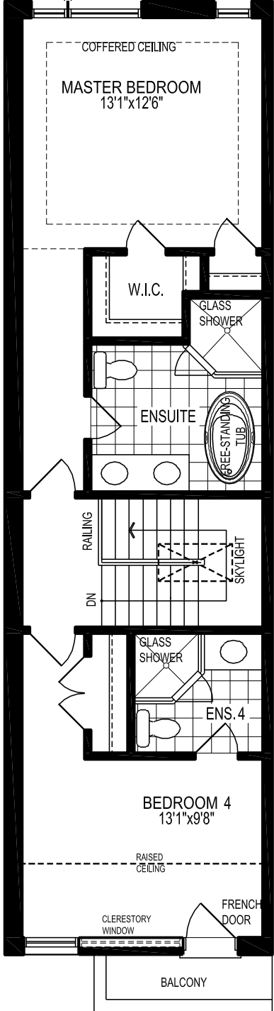
ALT. UPPER FLOOR PLAN 'A'
