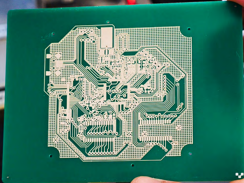
A 'graphical LCD and touchscreen overlay controller' printed and cured on an FR4 rigid substrate by the Voltera V-One.
