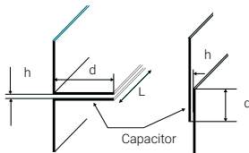
Figure 20 There should be a direct electrical connection to the enclosure wall. If it is a cable, an EMC gland should be used (see figure 12). If you were to allow the cable to pass the hole insulated while connecting the cable braid via a (long) cable, the loop formed by it would pick up electromagnetic energy (a common mode current) and it would be conducted over the braid to the inside of the enclosure.
