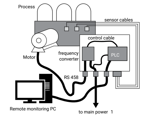
Figure 7 Several cable types can be observed in this diagram. It is usually helpful to draw a simplified diagram showing equipment as circles with interconnecting conductors. Do not forget to include power, "ground" and machine structure as conductors! In the diagram of figure 8, several cable types can be recognized.
