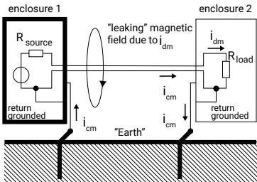
Figure 5 This alternative conductor could be the machine's structure, safety grounding provisions, the enclosure wall or other cables. This (induced) current in the usually larger loop is a common-mode (cm) current. Transfer impedance is a property of a complete interconnection: cable plus connectors, patch panels, etc. , from source to load. The properties of a very good cable can be ruined by a lousy finishing, e. g. , the infamous "pig-tail" construction on shielded cables.
