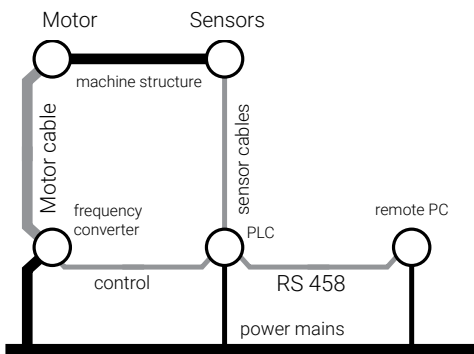
Figure 8 Cables with large and/or high frequency currents. Indicate this type using a red color or the letter "E" for Emission: due to transfer-impedance it will generate possibly large common mode currents.
