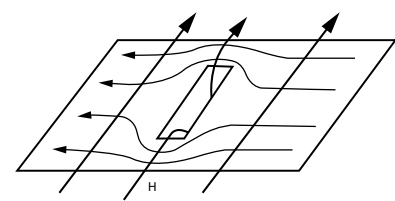
Figure 18 The effect of the field is a current in the shielding. This current generates a field which opposes the incident field. This way even non-magnetic materials can be used as shielding.
