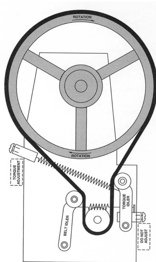
Fig. 18 Consistency Adjustment
