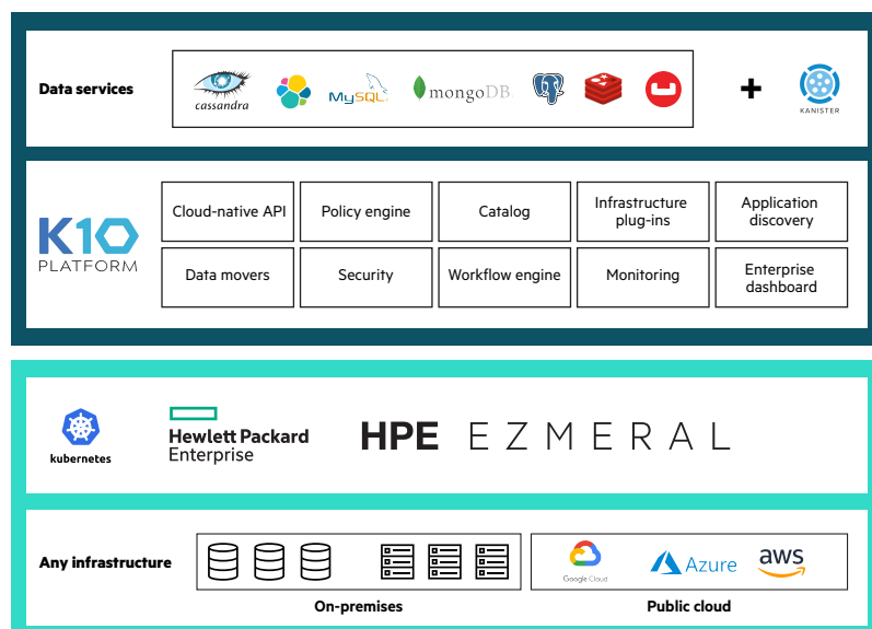
FIGURE 1. Kubernetes backup in HPE Ezmeral Container Platform with Kasten K10
