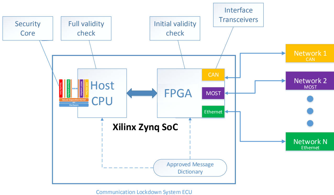
Figure 4: Communication Lockdown System ECU
