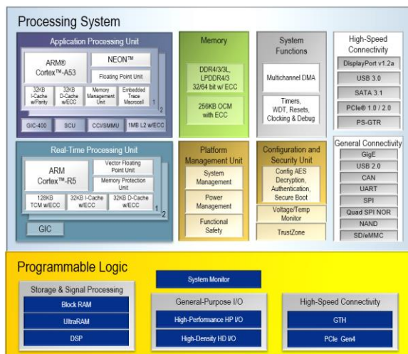
Figure 5: Zynq US+ MPSoC Partitioning: Processing System and Programmable Logic
