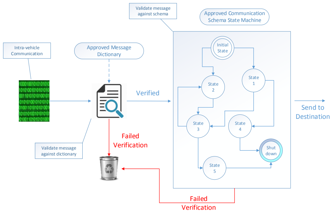
Figure 1: Communication Lockdown with State Machine
