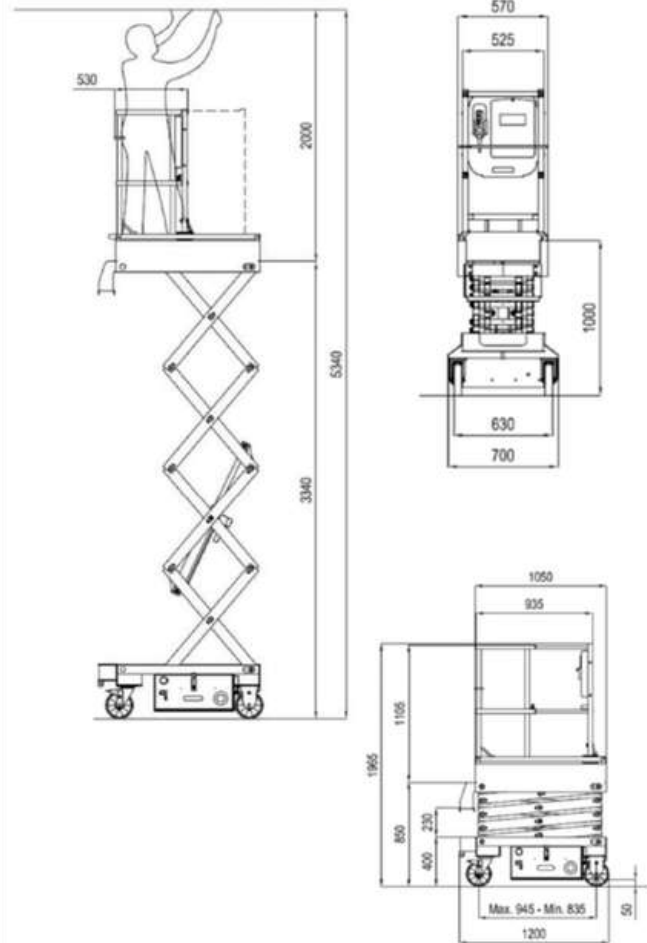
Push 5.3 Adjustable
