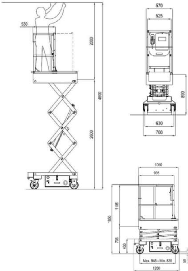
Push 4.6 Adjustable
