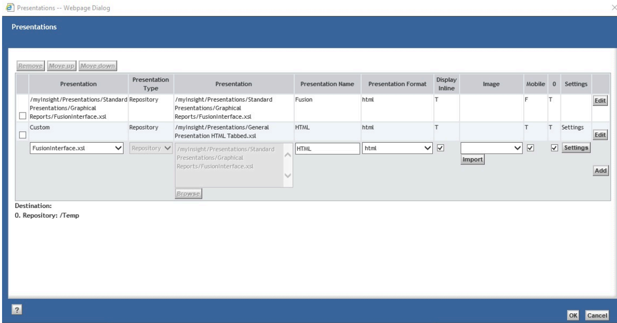
Figure 28: Presentation overview
