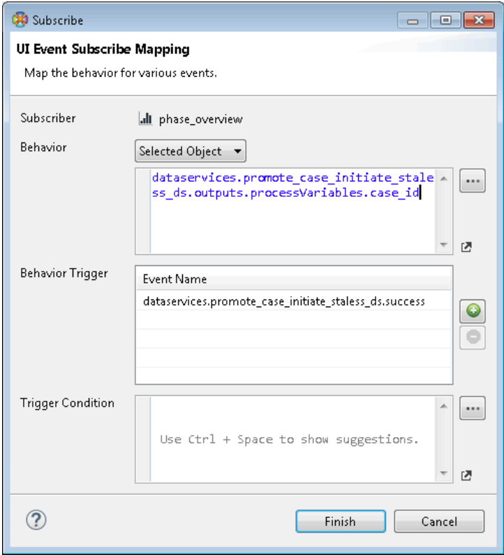
Figure 81: Using the returned Object ID
