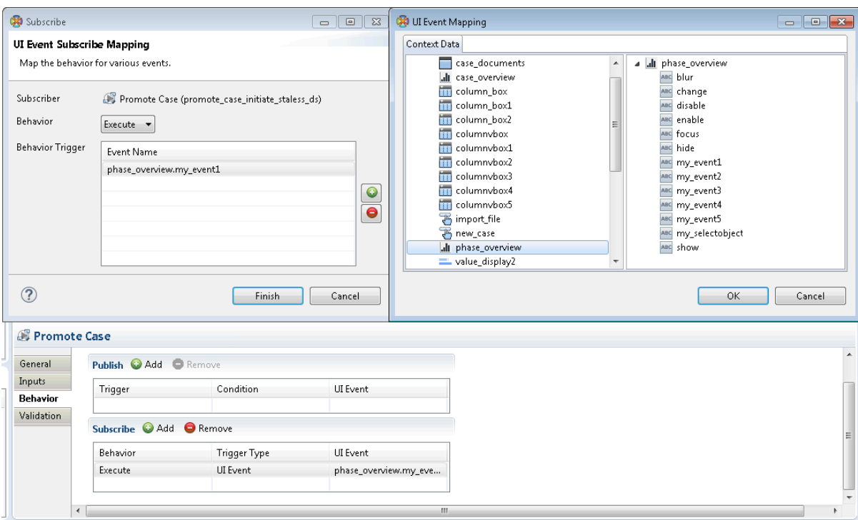
Figure 80: Registering a myInsight click event in xCP
