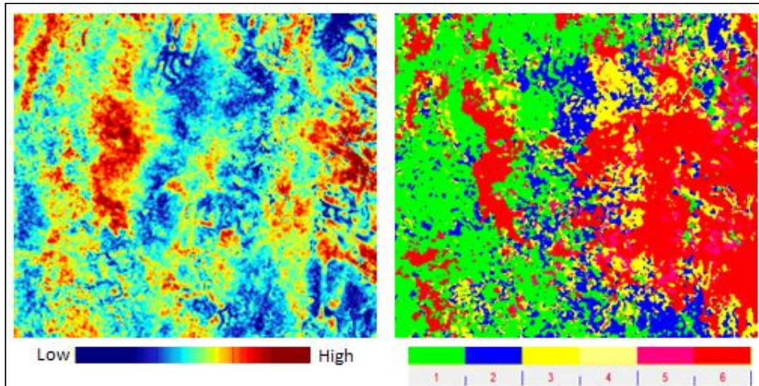
Figure 5: A horizon slice at the Evie Shale level from (left) the relative acoustic impedance volume derived from thin-bed reflectivity inversion of 3D seismic data, and (right) from waveform classification of a window extending 20 ms below the Evie-Shale marker. Notice the overall pattern of the red color seems to follow the pattern seen on the high impedance see on the left.
