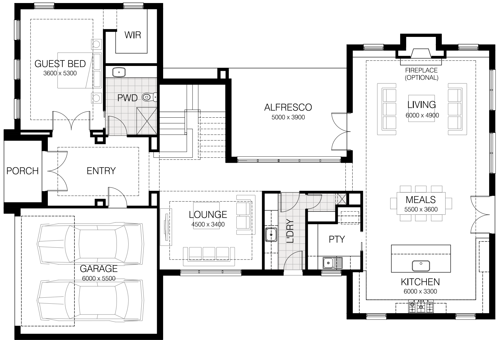
GROUND FLOOR
