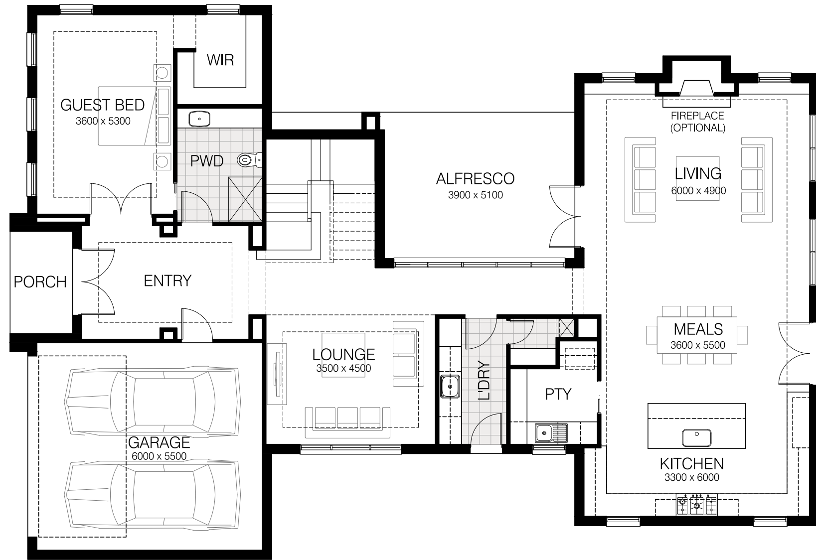
GROUND FLOOR
