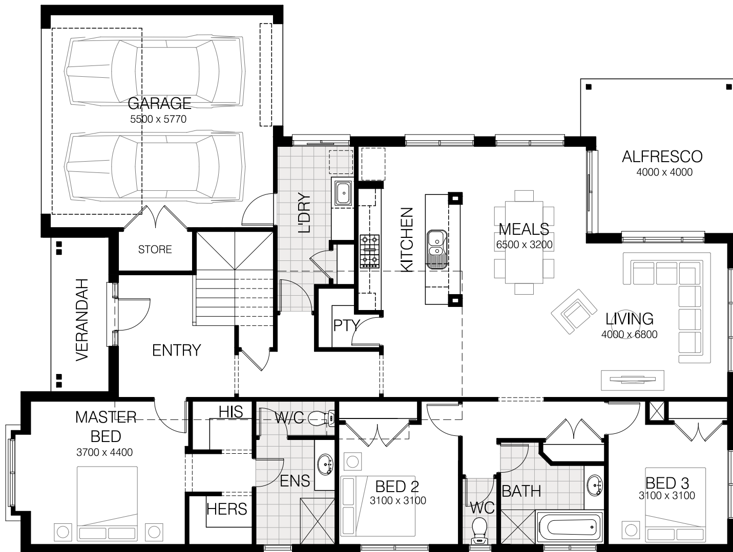
GROUND FLOOR
