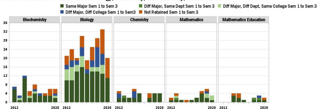
FIGURE 11: GRAPH OF RETENTION FROM 1 ST SEMESTER TO 3 RD SEMESTER IN DEPARTMENTS OF BIOLOGY, CHEMISTRY, AND MATHEMATICS
