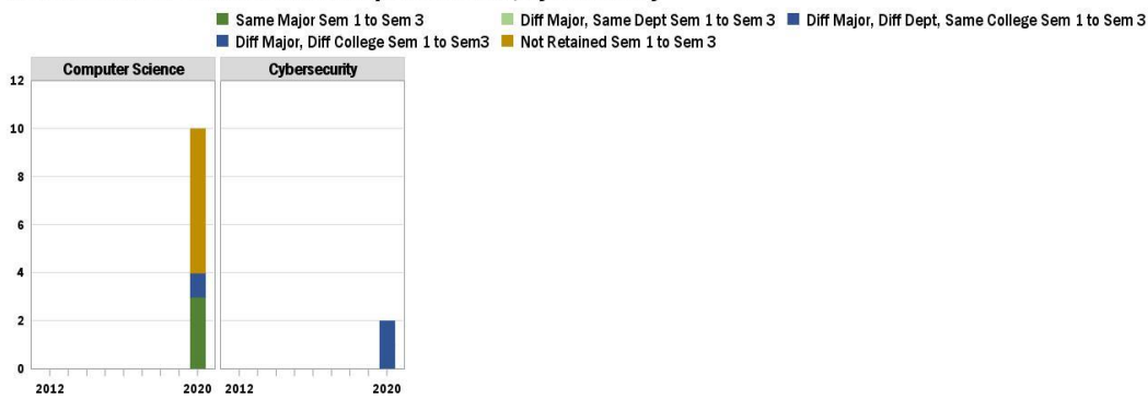
Retention 1st to 3rd Semester: Computer Science, Cybersecurity
