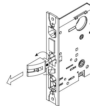
Change latch direction and secure with screw from countersink
